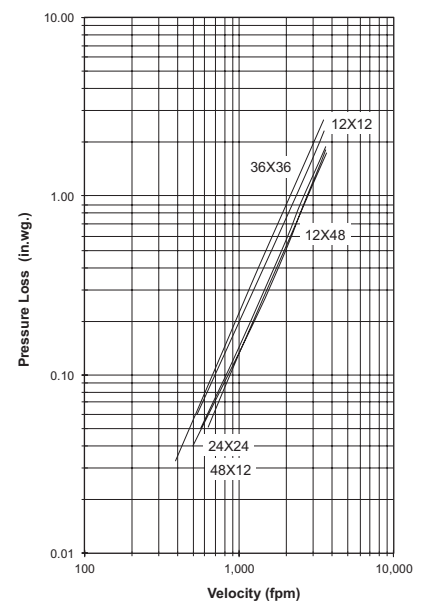
Figure 5.5 — Plenum Mount
