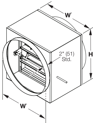
Sleeve Type R (Optional) Round duct transitions are standard with D=W=H . (available with D<W and H )
