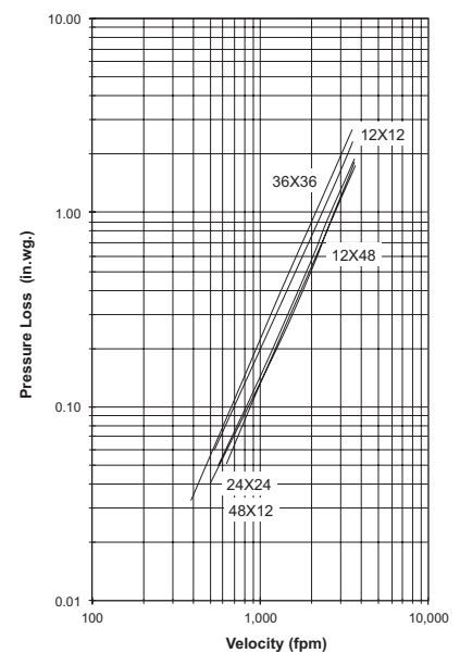
Figure 5.5 — Plenum Mount
