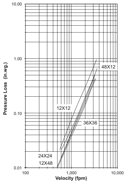
Figure 5.3 — Ducted Inlet and Outlet
