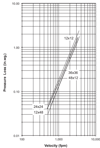
Figure 5.2 — Ducted Inlet
