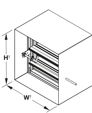
Sleeve (Optional)
