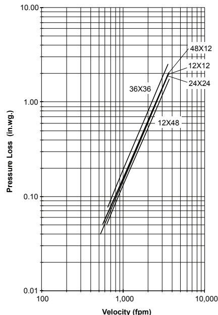
Figure 5.5 — Plenum Mount
