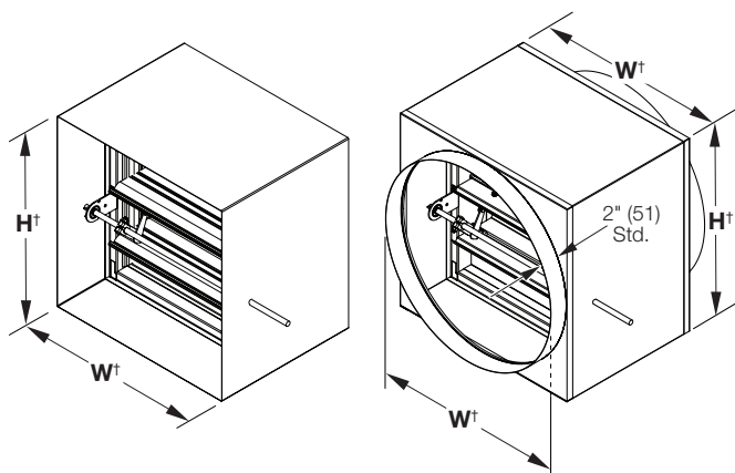
Sleeve (Optional)
