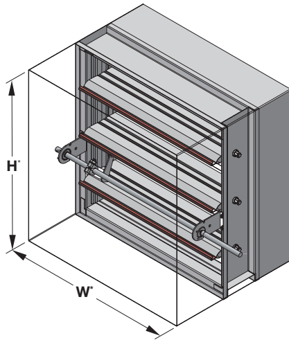
SD-181-SS (standard)
