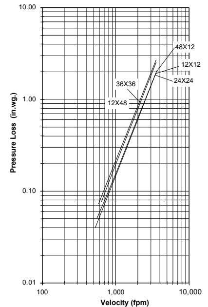
Figure 5.5 — Plenum Mount
