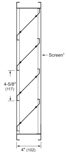
Vertical Section
