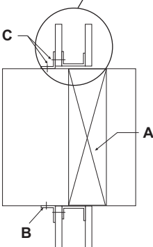
Figure 2: Metal Stud
