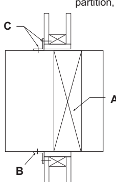
Figure 4: Wood Stud
