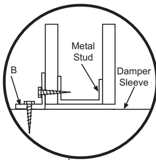
Single Mounting Angle Over Drywall
