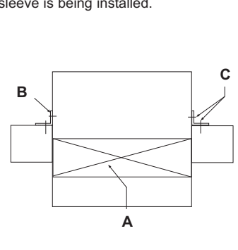
Figure 6: Horizontal Installation Concrete or Masonry only
