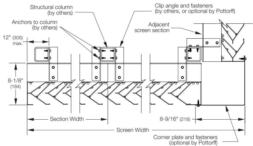
Horizontal Section
