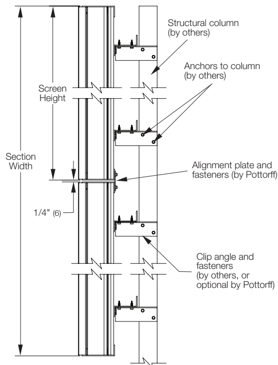
Vertical Section
