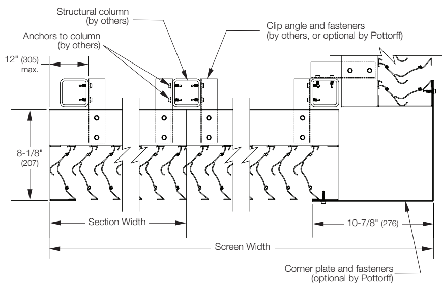
Horizontal Section
