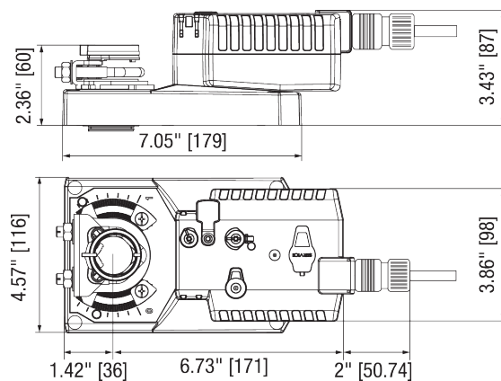
Dimensional drawings
